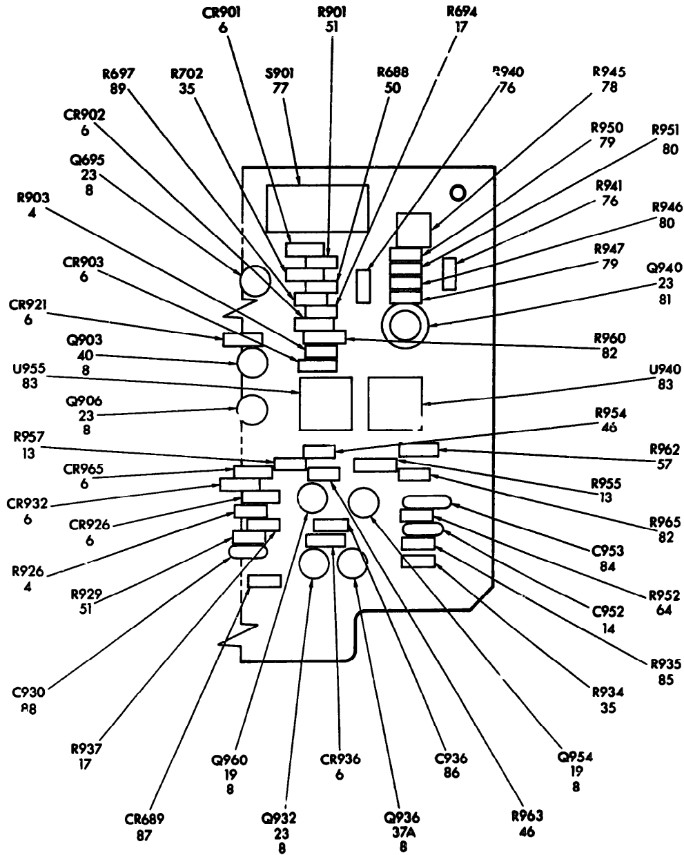
FIGURE 2-6. CIRCUIT CARD ASSEMBLY /A4/ /SHEET 4 OF 4/
