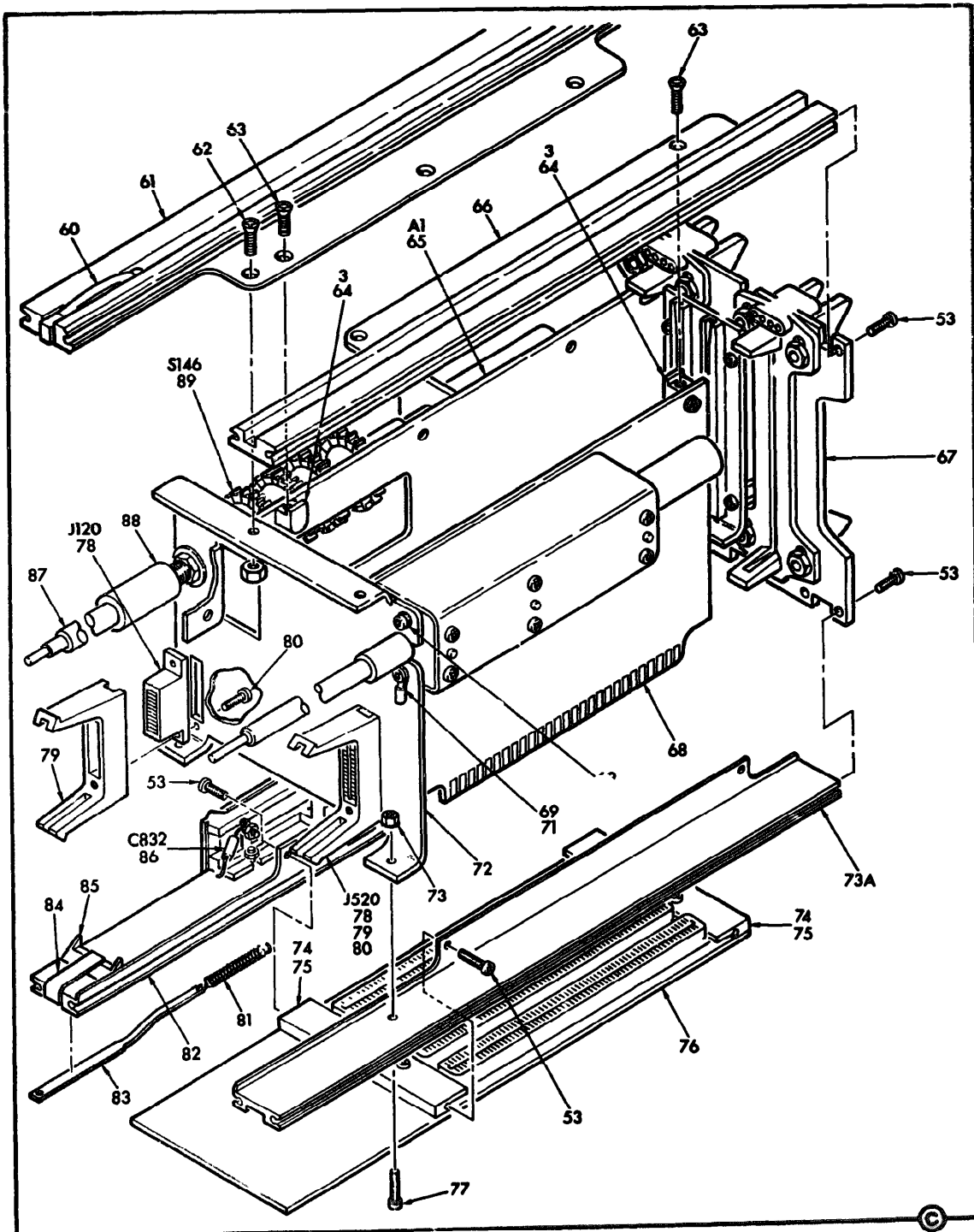
FIGURE 2-1. DUAL TIME BASE PLUG-IN TO-1160/P/U// SHEET 3 OF 3/
