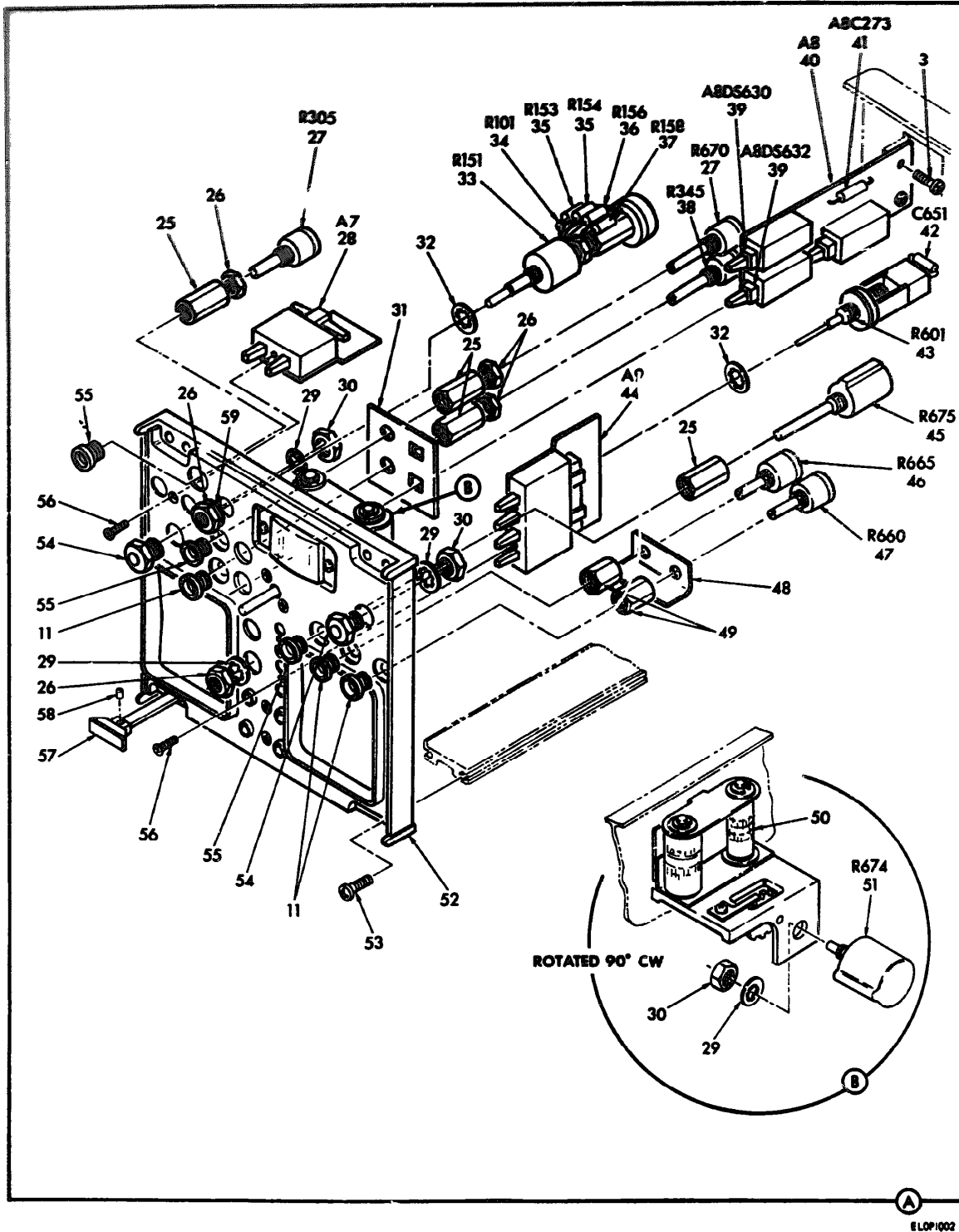
FIGURE 2-1. DUAL TIME BASE PLUG-IN UNIT TD-1160/P/U/ /SHEET 2 OF 3/
