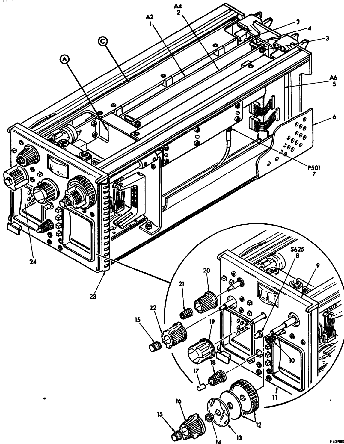
FIGURE 2-1. DUAL TIME BASE PLUG-IN UNIT TD-1160/P/U/SWEET 1
