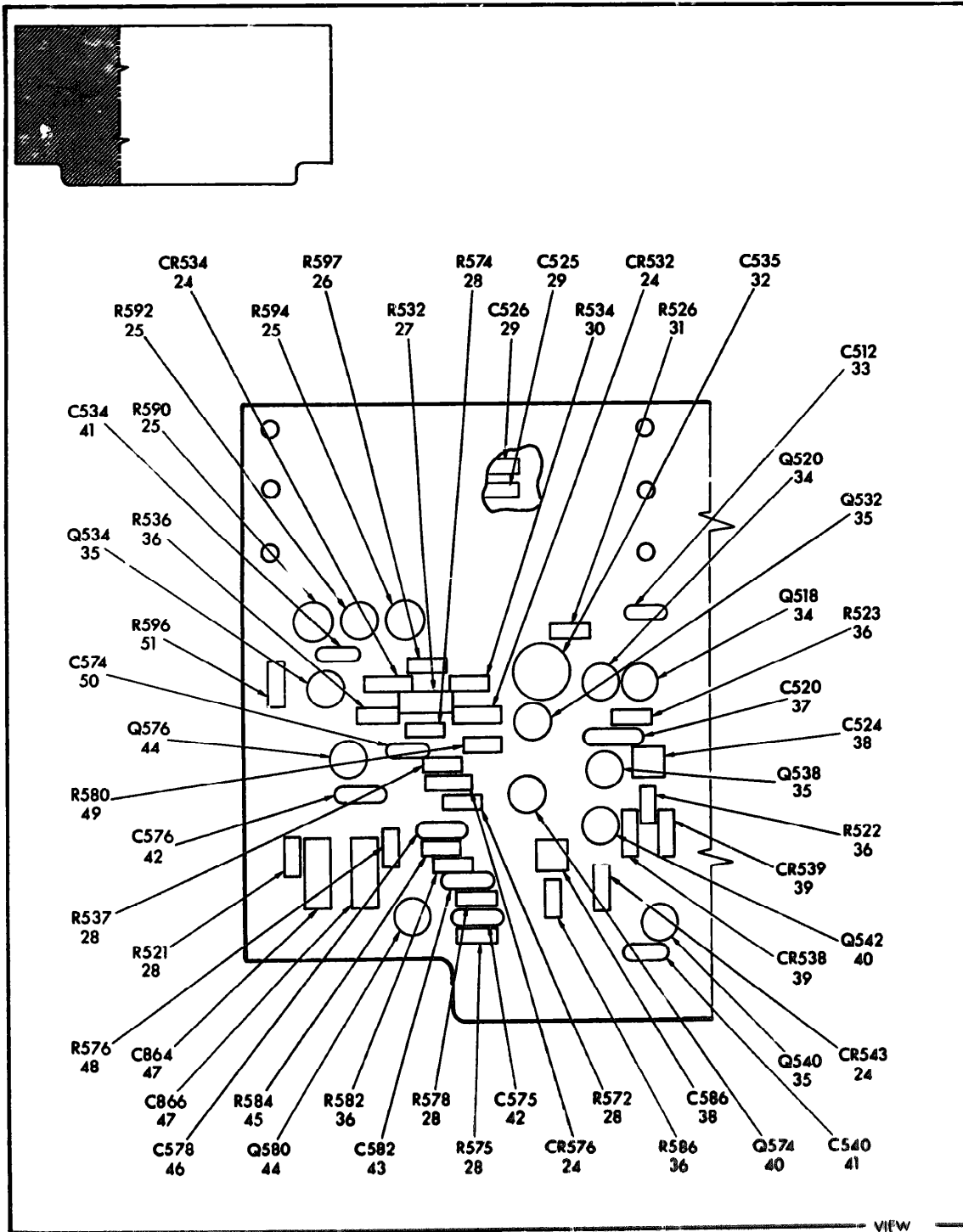
FIGURE 2-4. CIRCUIT CARD ASSEMBLY /A3/ /SHEET 2 OF 4/
