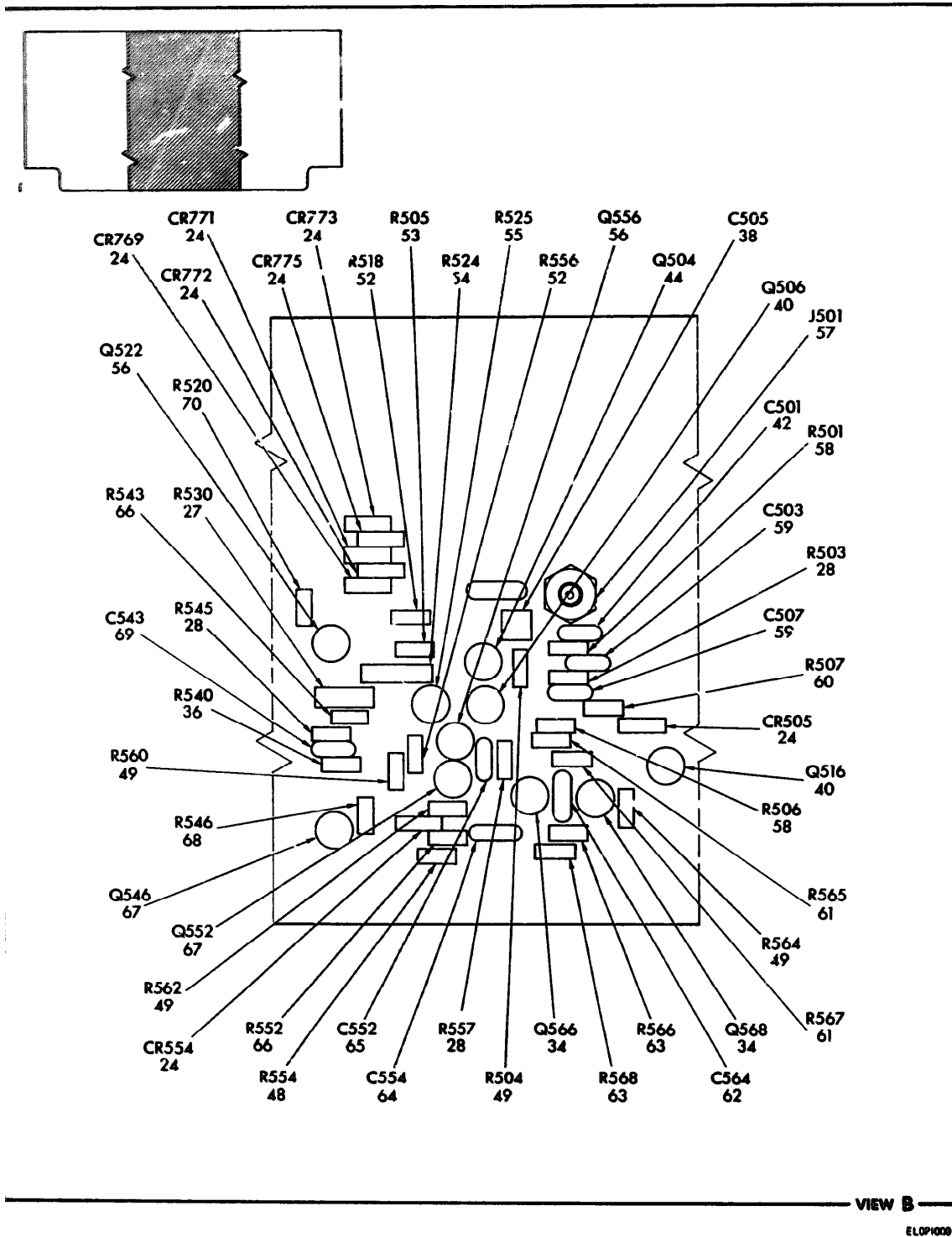
FIGURE 2-4. CIRCUIT CARD ASSEMBLY /A3/ /SHEET 3 OF 4/
