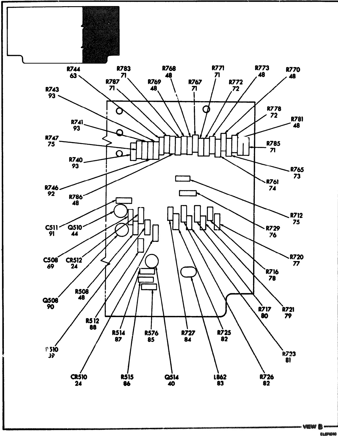
FIGURE 2-4. CIRCUIT CARD ASSEMBLY /A3/ /SHEET 4 OF 4/
